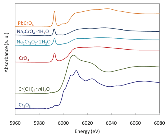
Figure 1. XANES K-edge spectra for \text{Cr}_2\text{O}_3 , \text{Cr}(\text{OH})_3 \cdot n\text{H}_2\text{O} , \text{CrO}_3 , \text{Na}_2\text{Cr}_2\text{O}_7 \cdot 2\text{H}_2\text{O} , \text{Na}_2\text{CrO}_4 \cdot 4\text{H}_2\text{O} , and \text{PbCrO}_4 . The spectra are vertically deviated for clarity.
