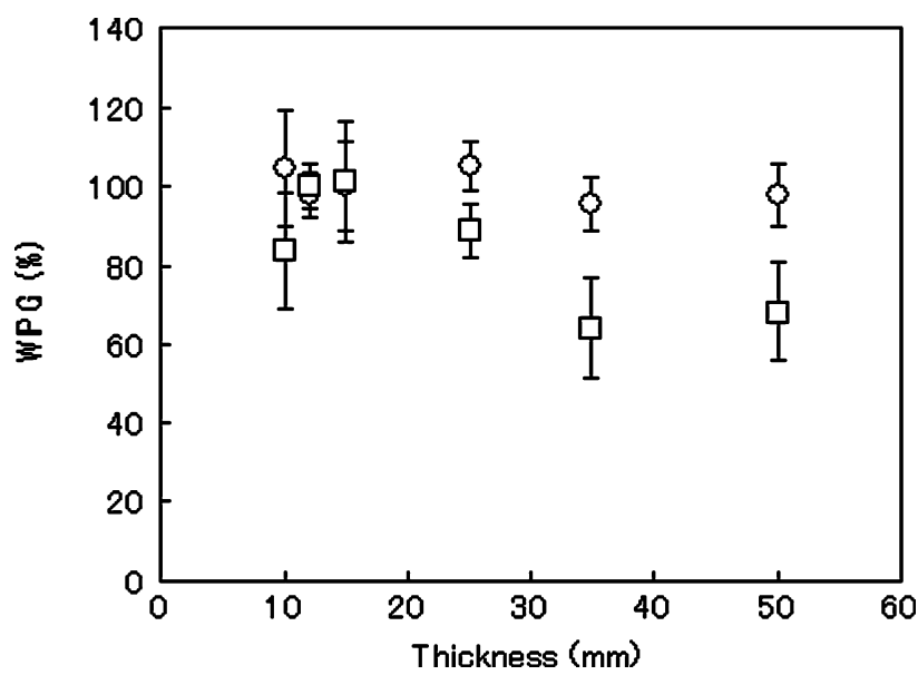
Figure 2. Comparison of permeability of laminated wood ○, and solid wood □, with different thickness. The error bars denote standard deviation (n = 12).
